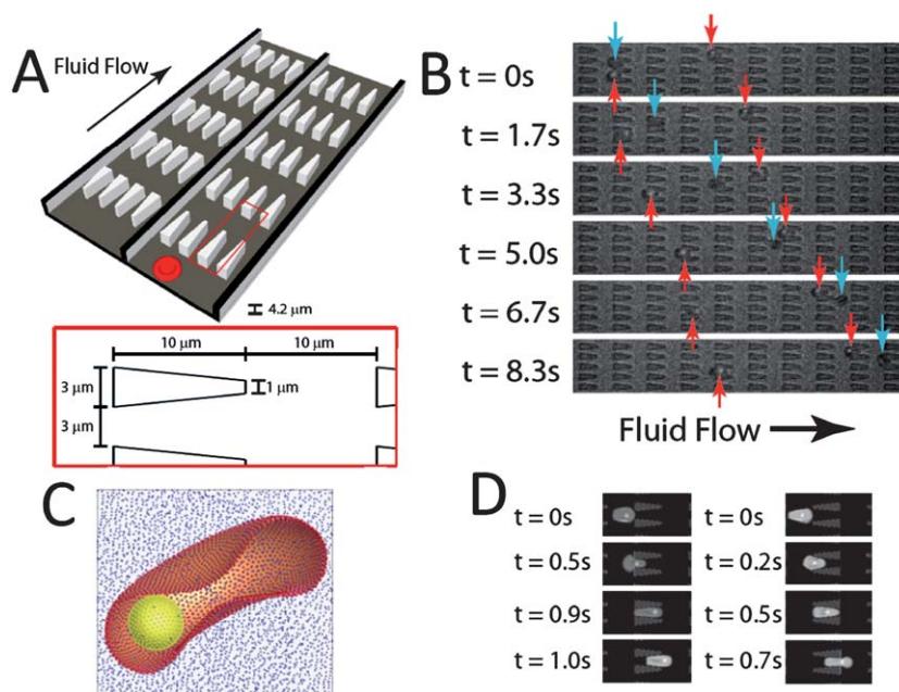
Fig. 1 A) Illustration of the device design; each channel of the actual device is 10 pores wide and 200 pores long. (B) Experimental images of ring stage P. falciparum -infected (red arrows) and uninfected (blue arrows) RBCs in the channels at a pressure gradient of 0.24 \text{ Pa } \mu\text{m}^{-1} . The small fluorescent dot inside the infected cell is the GFP-transfected parasite. At 8.3 s, it is clear that the uninfected cell moved about twice as far as each infected cell. (C) The computational RBC model consists of 5000 particles connected with links. The P. falciparum parasite is modeled as a rigid sphere inside the cell. (D) DPD simulation images of P. falciparum -infected RBCs traveling in channels of converging (left) and diverging (right) pore geometry at 0.48 \text{ Pa } \mu\text{m}^{-1} .
