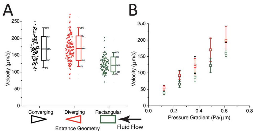
Fig. 2 A) Velocity of individual 200 nm diameter beads at a pressure difference of 0.49 \text{ Pa } \mu\text{m}^{-1} . There is no statistically significant difference in the velocity of beads travelling through the converging and diverging geometries. The beads travelling through the channel with rectangular obstacles move slower on average. (B) Velocity vs. pressure for the different obstacle geometries.
